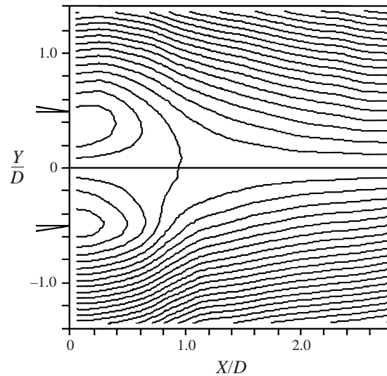
FIGURE 6. Streamline pattern of the wake flow behind a flat plate with base suction speed U_s/U_\infty = 0.5 and Re = 1000 , U = 10.0 \text{ cm s}^{-1} . It was computed by a mass balance from the velocity flow field shown in figure 5.
