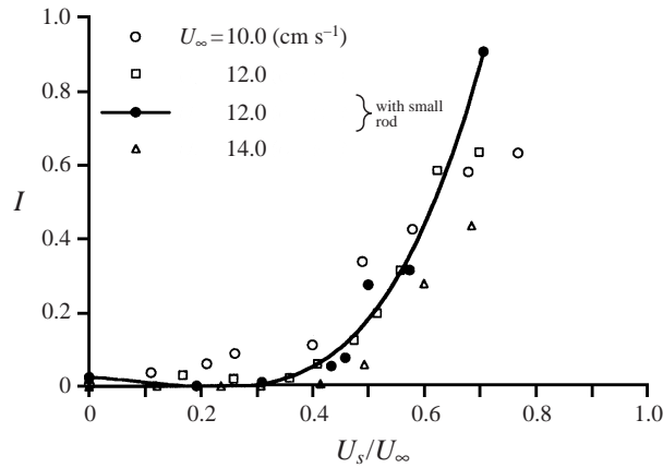
FIGURE 14. Stable intermittency I as function of suction speed ( U_s/U_\infty ) at free-stream velocities U_\infty = 10 \text{ cm s}^{-1} ( Re = 1000 ), U_\infty = 12 \text{ cm s}^{-1} ( Re = 1200 ), and U_\infty = 14 \text{ cm s}^{-1} ( Re = 1400 ).
