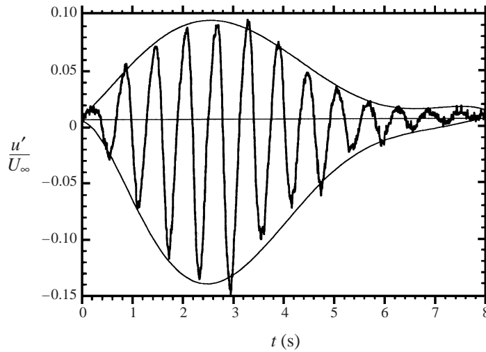
FIGURE 21. Impulse train response of U -velocity fluctuation at (X/D, Y/D) = (3.0, 0.5) for the plane wake flow at Re = 1600 with suction U_s/U_\infty = 0.75 and five transverse pulses by oscillating a rod at 1.7 Hz amplitude of 0.05D .
